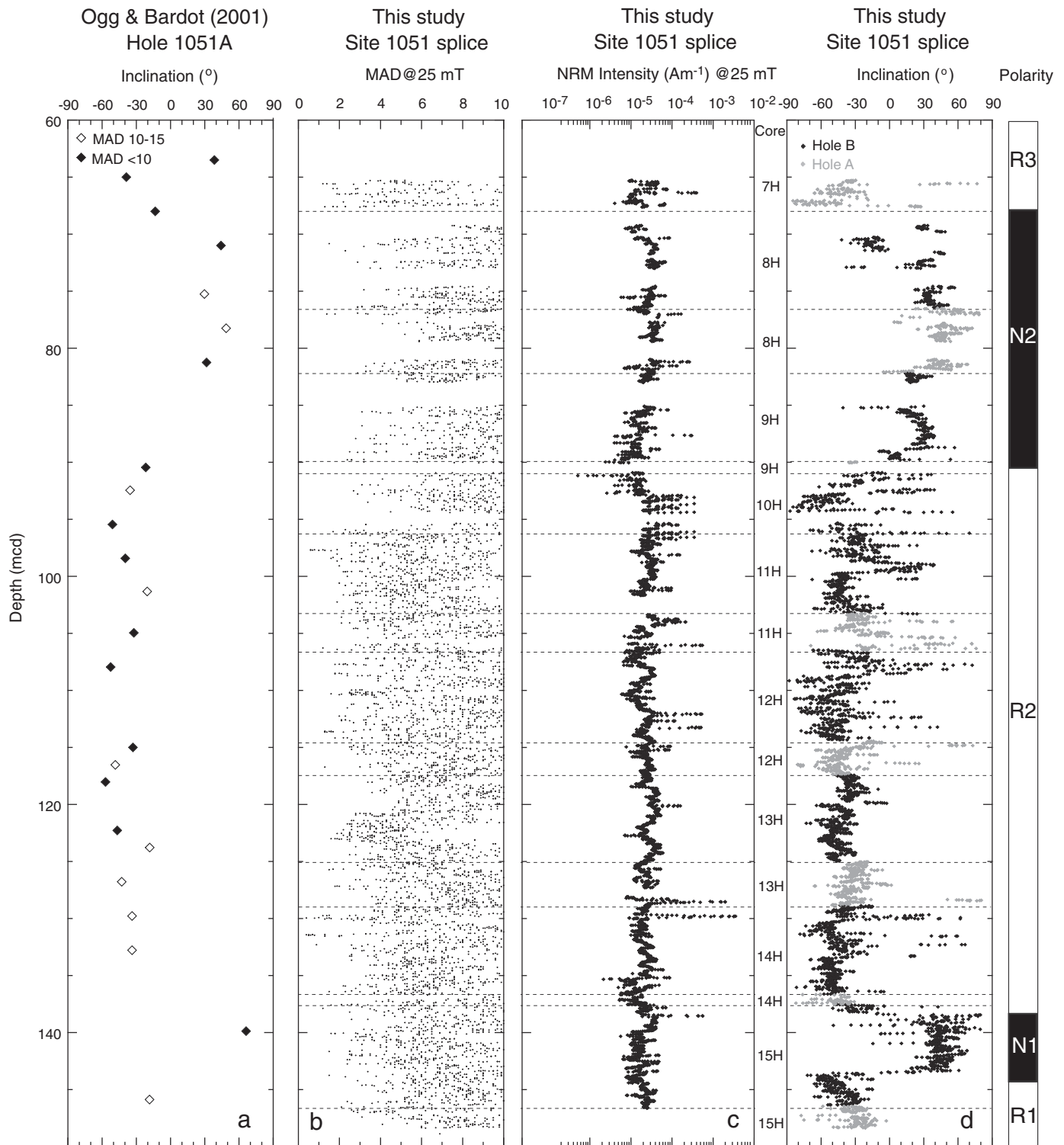
Fig. 4. Down-core variations in the intensity of the natural remanent magnetization (NRM) and inclination for ODP Site 1051. a) Inclination data from Ogg and Bardot (2001) . Closed symbols represent data points with maximum angular deviation (MAD) values of <10^\circ , while open data points have MAD values between 10^\circ and 15^\circ . b) MAD values of data shown in panels c and d. c) NRM intensity after AF demagnetization at 25 mT for samples shown in panel c. d) Inclination data for the shipboard composite depth sections (mcd – meters composite depth). Grey symbols = data from Hole A and black symbols from Hole B, with MAD values of <10^\circ (this study). Horizontal dashed lines represent splice points. The magnetic polarity zonation is shown on the right. Black represents normal and white represents reversed polarity intervals.
