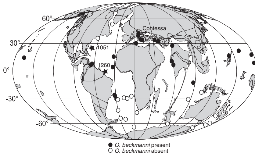
Fig. 2. Palaeogeographic reconstruction of the Eocene illustrating the presence and absence of Orbulinoides beckmanni . ODP Sites 1051 and 1260 (stars) used in this study. Solid circles indicate the presence and open circles the absence of O. beckmanni . Data are compiled from deep-sea drill sites and exposed marine sections that coincide with planktonic foraminiferal Zone E12 but are not necessarily stratigraphically 'complete' sections. Data are compiled from Lowrie et al. (1982), BouDagher-Fadel and Clark (2006), Premoli Silva et al. (2006), Babic et al. (2007), Jovane et al. (2007) and http://www-odp.tamu.edu/database/ . To prevent bias, sites where O. beckmanni is absent because of hiatuses, dissolution, lack of carbonate or non-recovery of this stratigraphic interval are excluded. The base map for 40 Ma was generated from http://www.odsn.de/odsn/series/palaeomap/palaeomap.html .
