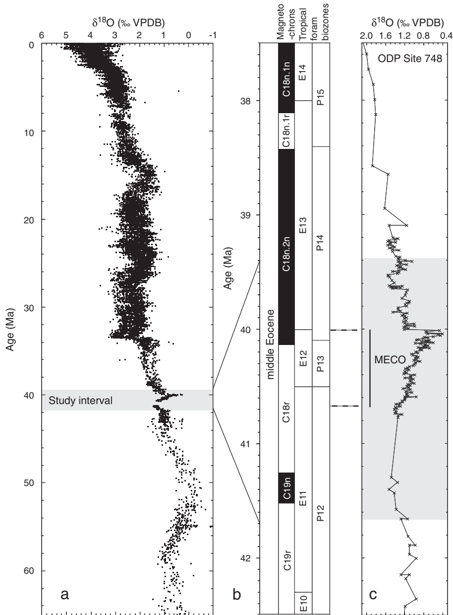
Fig. 1. Study interval in the context of Cenozoic climate trends. a) Cenozoic benthic foraminiferal \delta^{18}\text{O} record modified from Zachos et al. (2008). The MECO is shown on a revised age scale in keeping with this study. b) The Geomagnetic polarity time scale used follows Cande and Kent (1992; 1995). New 'E' planktonic foraminiferal tropical biozonation scheme from Berggren and Pearson (2005), and 'P' tropical biozonation scheme from Berggren et al. (1995). c) Benthic foraminiferal \delta^{18}\text{O} record from Site 748, Southern Ocean (Bohaty et al., 2009). Black vertical line represents the duration of the MECO based on the \delta^{18}\text{O} stable isotope pattern. Black dashed lines denote the position of the MECO relative to the GPTS and tropical zonation scheme. Grey boxes denote the study interval and the black vertical line represents the duration of the MECO based on the \delta^{18}\text{O} pattern.
