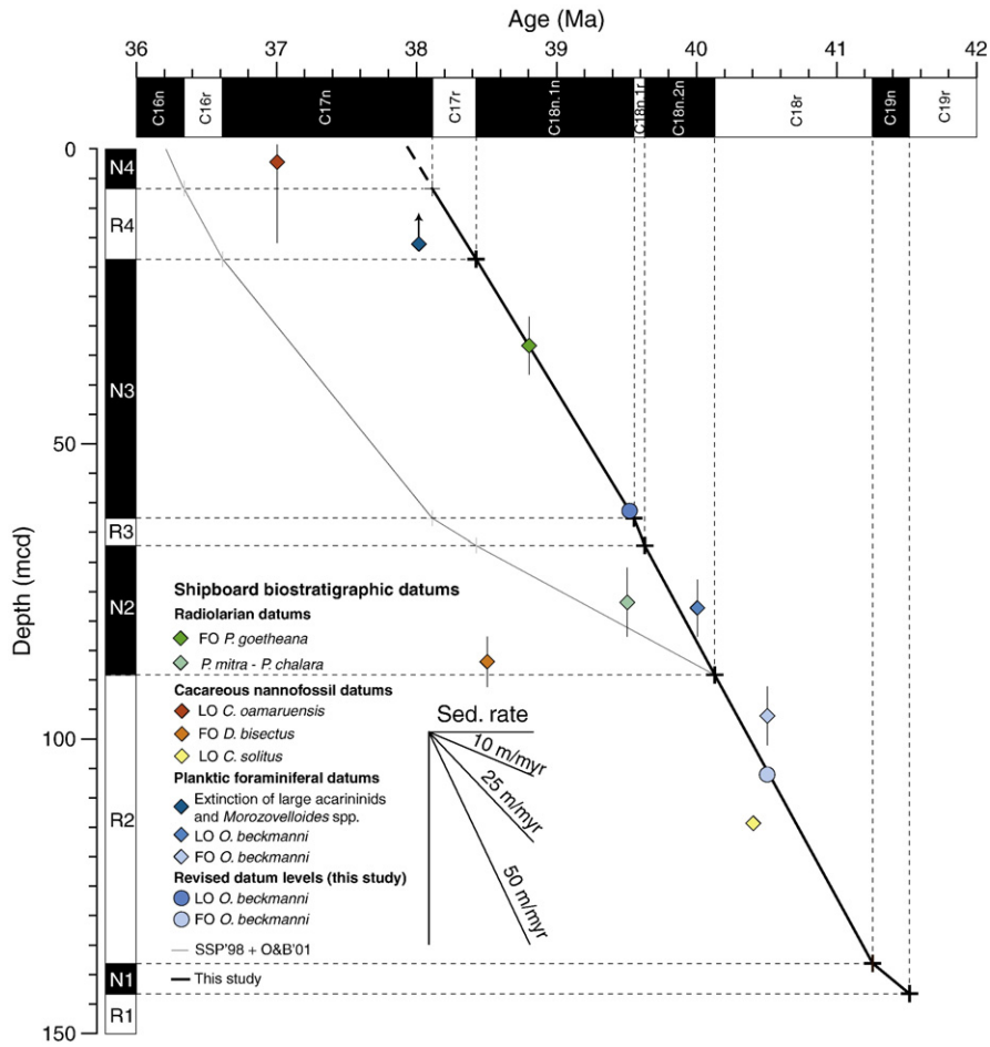
Fig. 6. Age versus depth plot with correlation of the ODP Site 1051 polarity zonation to the geomagnetic polarity time scale of Cande and Kent (1992, 1995). Calcareous plankton and radiolarian datums determined by the Shipboard Scientific Party (1998) are shown by colored diamonds (errors indicated by vertical black lines). Ages are from Berggren et al. (1995), with the exception of the highest occurrence (HO) of O. beckmanni and the extinction of Morozovelloides and large acarininids, which are from Wade (2004). Revised placement of the LO and HO of O. beckmanni are shown by solid circles. Polarity intervals marked 'R' have reversed polarity and those marked 'N' have normal polarity. mcd = metres composite depth. The grey line represents the age model from SSP'98 = Shipboard Scientific Party (1998) and O&B'01 = Ogg and Bardot (2001).
