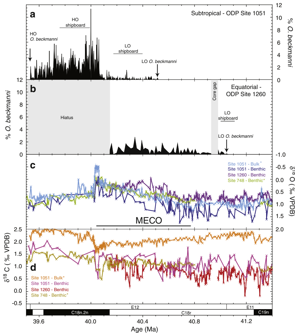
Fig. 5. Stable isotope records across the middle Eocene climatic optimum and relative abundance records of O. beckmanni . Relative abundance records of O. beckmanni at ODP Sites 1051 (panel a) and 1260 (panel b). Horizontal black lines denote core depths between which the lowest and highest occurrences (LO and HO) of O. beckmanni were recorded by the Shipboard Scientific Party (1998, 2004) Revised planktonic foraminiferal zone boundaries based on this study shown. Arrows indicate new placement of the boundaries of Zone E12. c) Benthic foraminiferal \delta^{18}\text{O} records from Sites 1051 and 1260 (this study). Starred (*) records are from Bohaty et al. (2009) and are aligned on the new Site 1051 age model. d) Benthic foraminiferal \delta^{13}\text{C} records from Sites 1051 and 1260 (this study). Starred (*) records are from Bohaty et al. (2009) and are aligned on the new Site 1051 age model.
